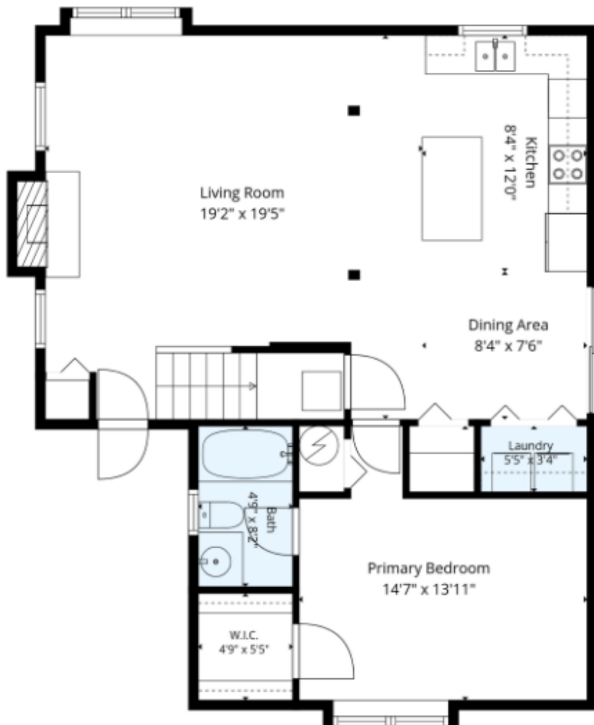
1st Floor
